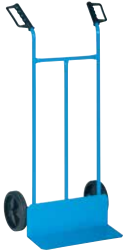
● MG408 Carrello portapacchi. Ruote in nylon gommato Ø 200 mm. Dim. pala mm.450x155 Portata kg. 200. Trolley for packs. Wheels made of rubberised nylon Ø 200. Shovel size mm450x155 Capacity kg. 200 | Diable tube d'acier. Roues nylon caoutchouté diam. 200 mm Dim. Bavette mm 450x155 charge kg. 200 l. 500 / p. 380 / h. 1100
